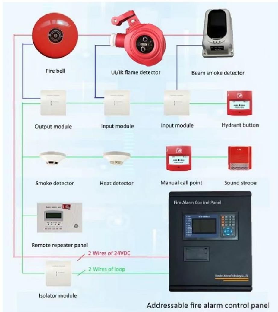
Wiring diagram of detector
